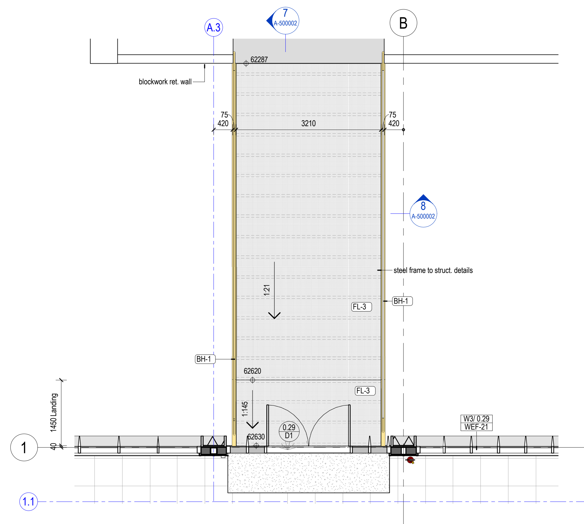
6 North Entry Link 1 : 50
