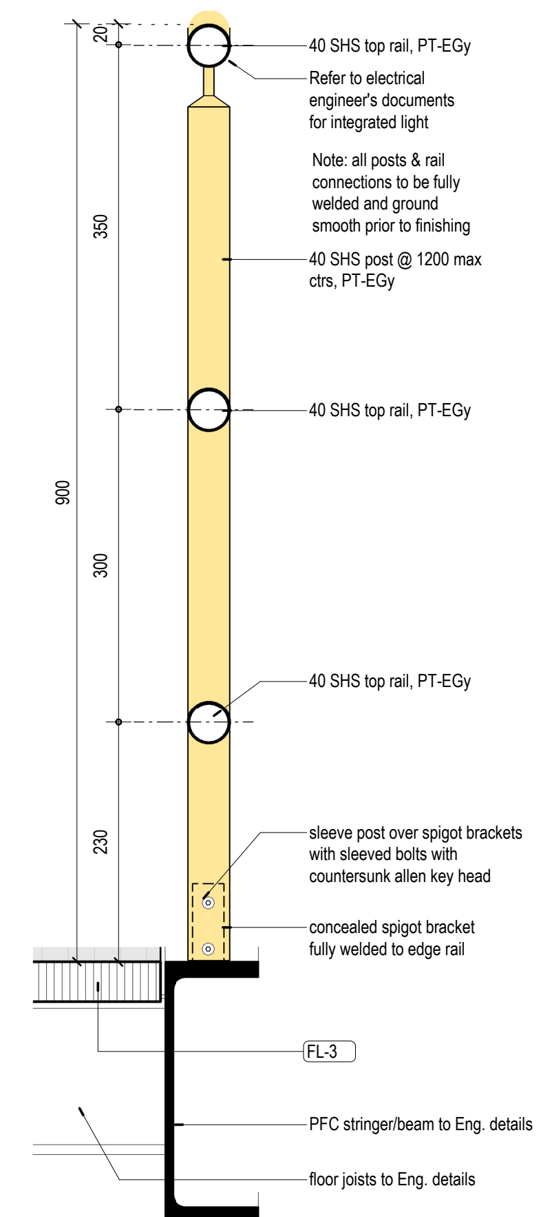
9 Entry Walkway - Section 1 1:5
