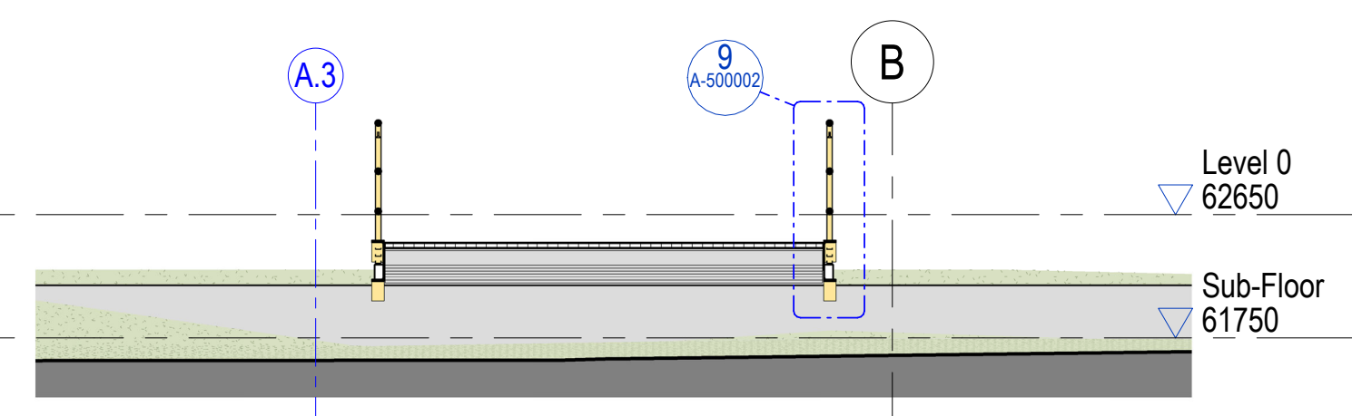
8 North Entry Link - Section 2 1 : 50
