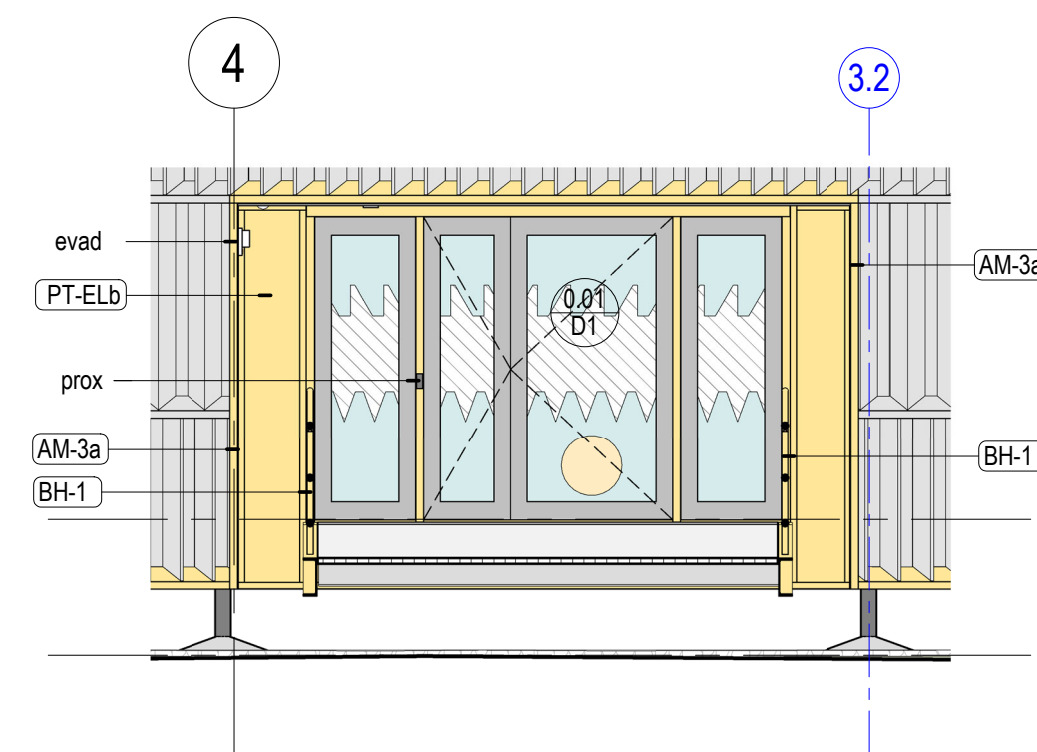
2 East Entry Walkway - Section 1 1:50
