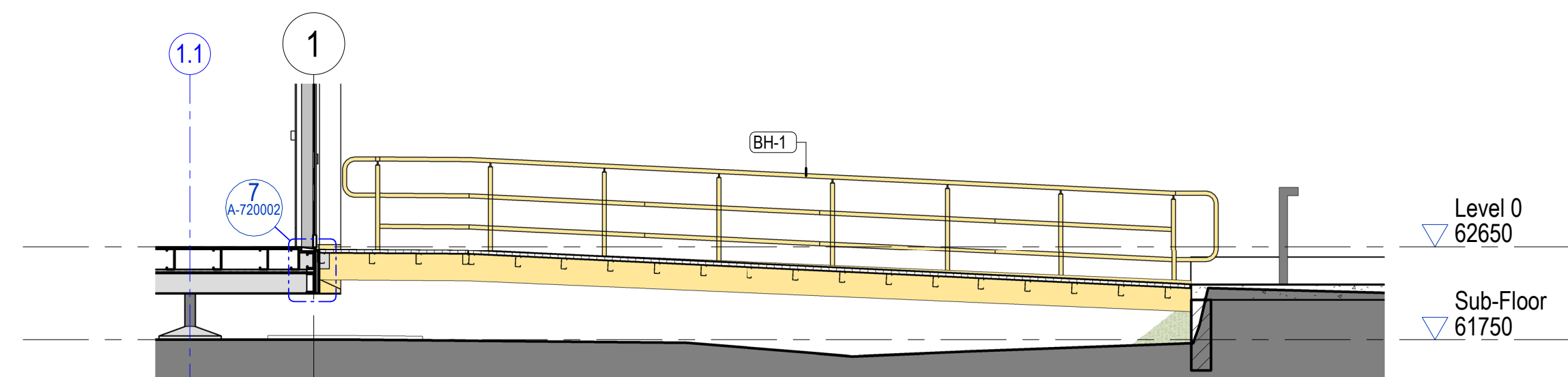
7 North Entry Link - Section 1 1 : 50
