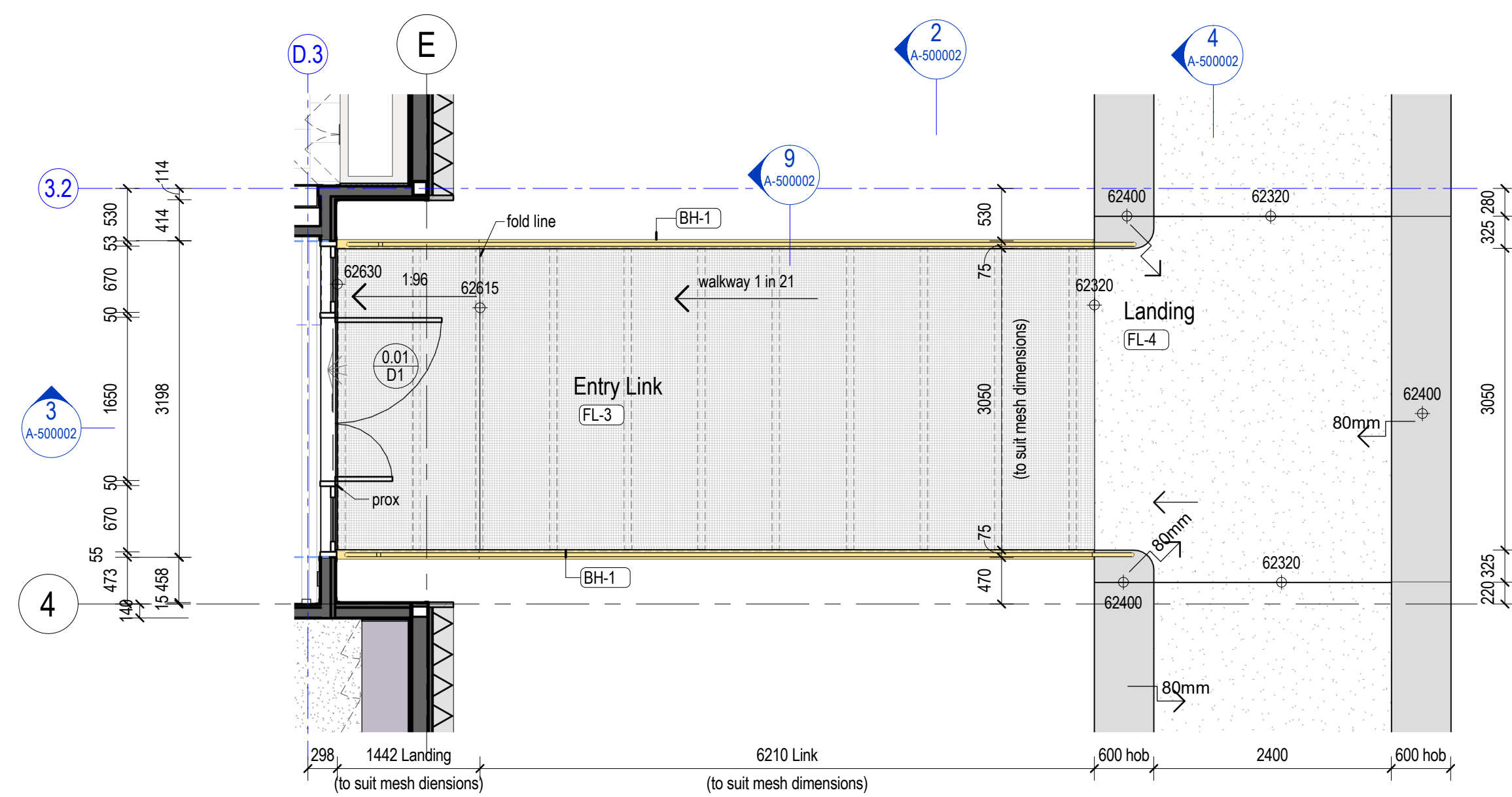
1 East Entry Walkway Link 1:50
