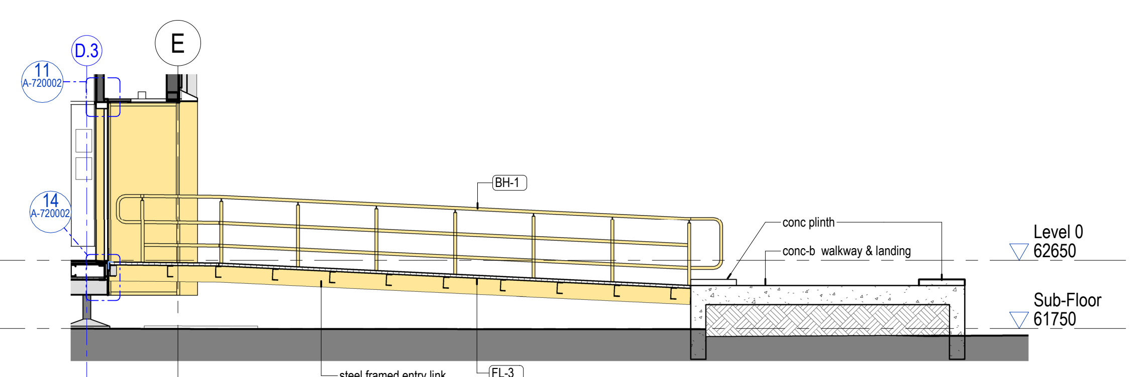
3 East Entry Walkway - Section 2 1 : 50
